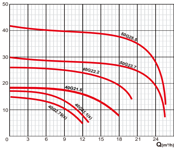
H(m) PERFORMANCE CHART AT n=3450min -1
