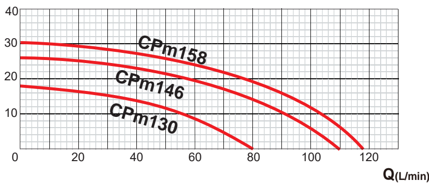
H(m) PERFORMANCE CHART AT n=3450min -1
